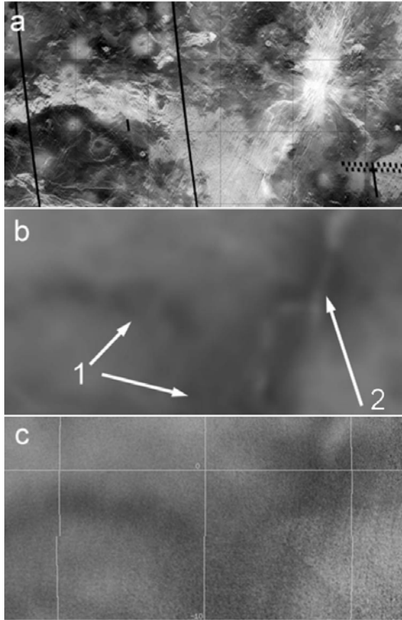
Figure 1. 1400 x 2800 km area centered at 4^{\circ}\text{N} 280^{\circ}\text{E} , 1 – tesserae, 2 – rifts. a) Magellan SAR image, b) model black body emission, c) VMC.
